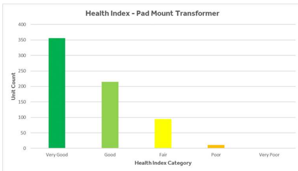
Figure 3-15: Underground Transformer Health Index Demographic
