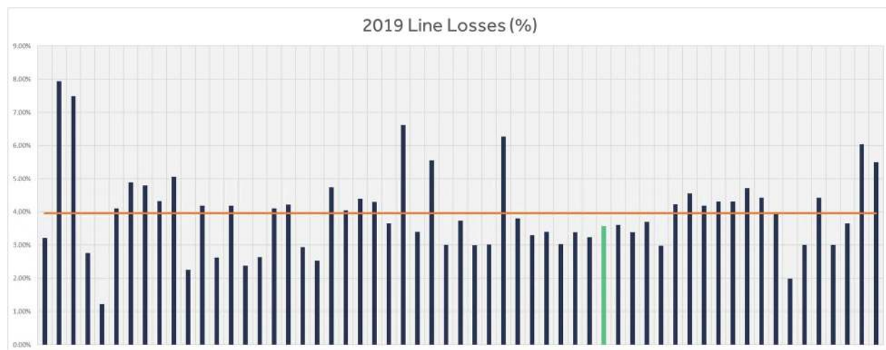
Figure 2-11: 2019 OEB Yearbook of Ontario Electricity Distributors Average Annual Line Loss
