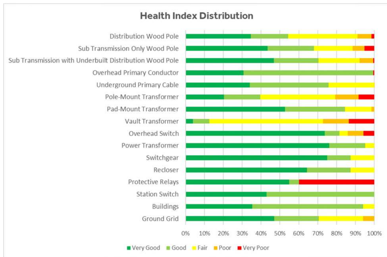
Figure 3-5: NBHDL Health Index Distribution for Major Assets
