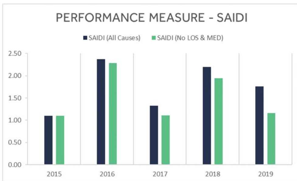
Figure 2-1: Performance Measure - SAIDI
