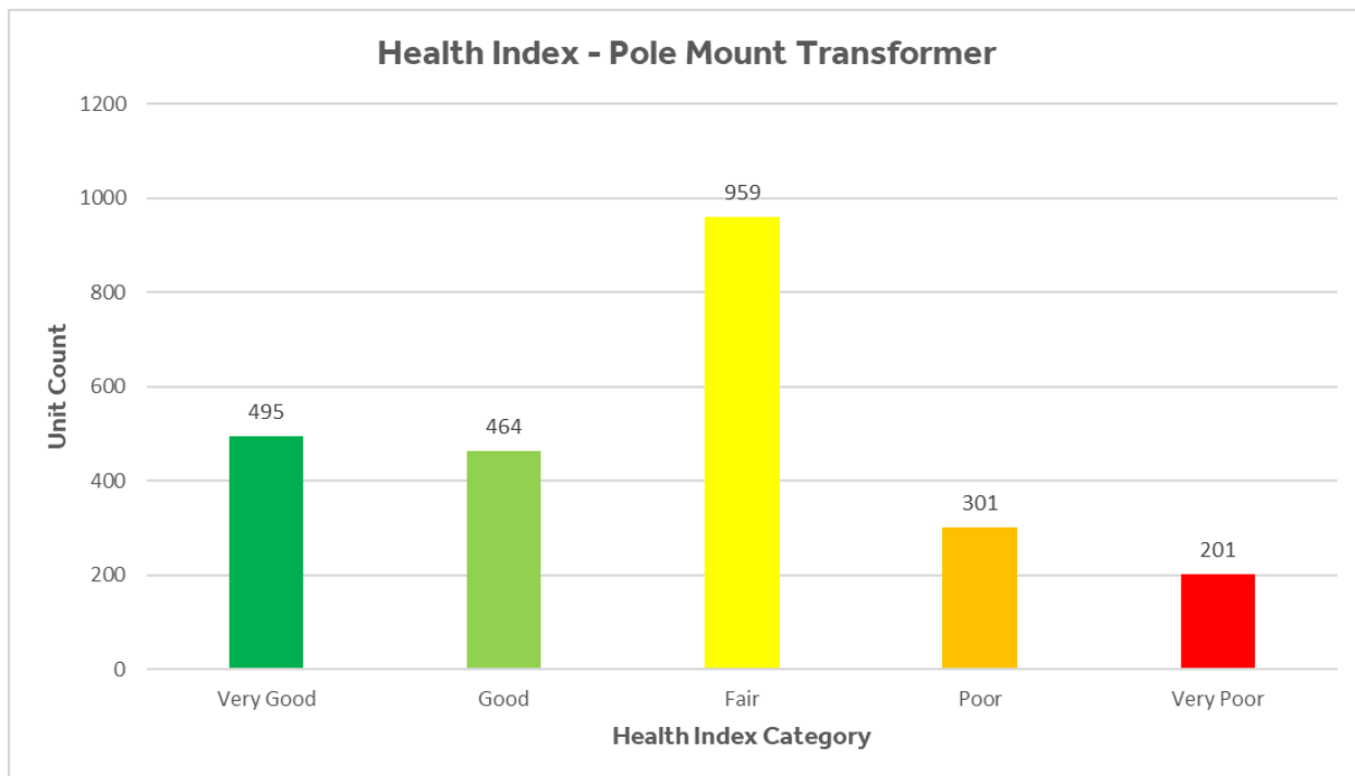
Figure 4-10: Pole-Mount Transformers Health Index Demographic
