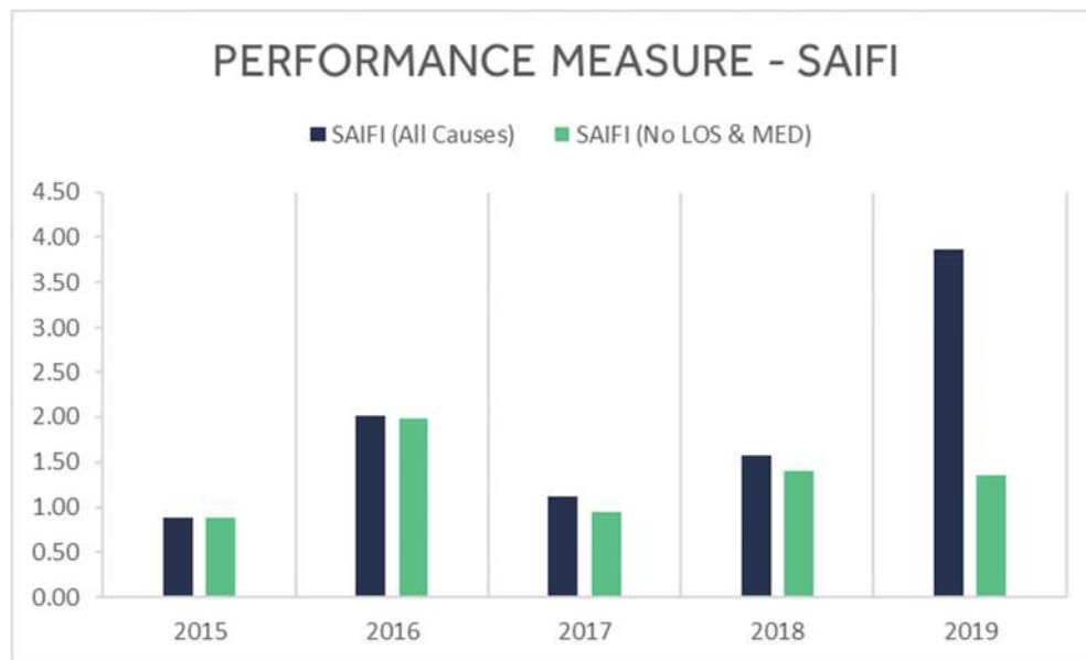
Figure 2-2: Performance Measure - SAIFI
