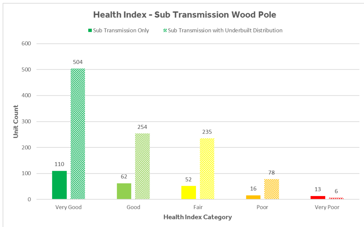
Figure 4-4: Sub-Transmission Wood Poles Health Index Demographic
