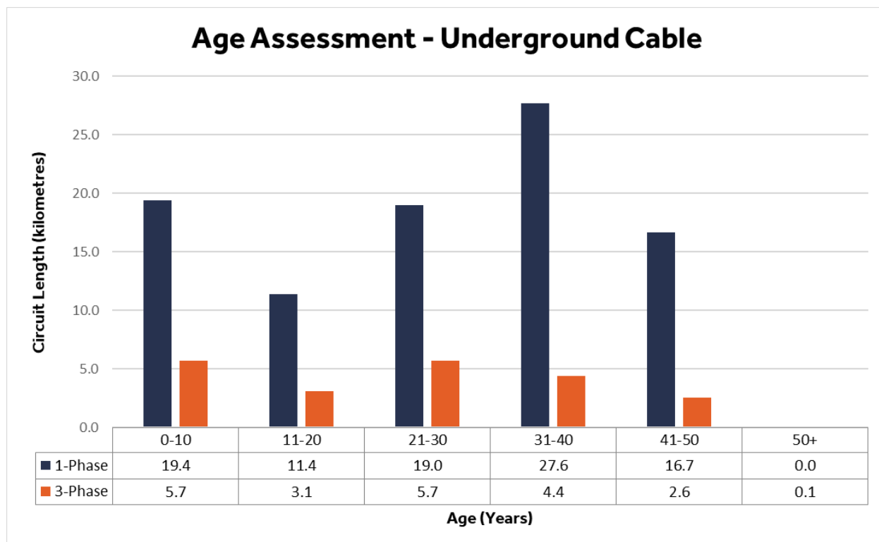
Figure 4-7: Overall Underground Primary Cable Age Demographic
