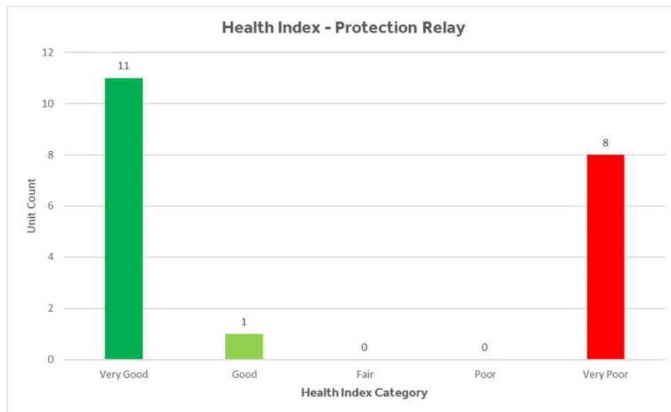
Figure 3-9: Protection Relay Health Index Demographic
