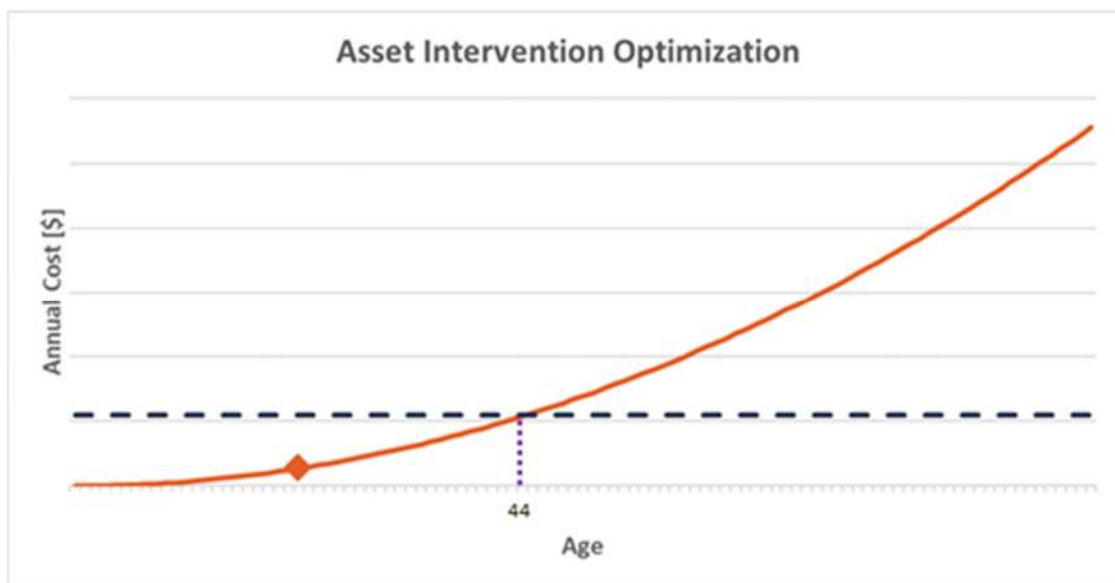
Figure 3-17: Asset intervention optimization strategy (example shown for power transformer)
