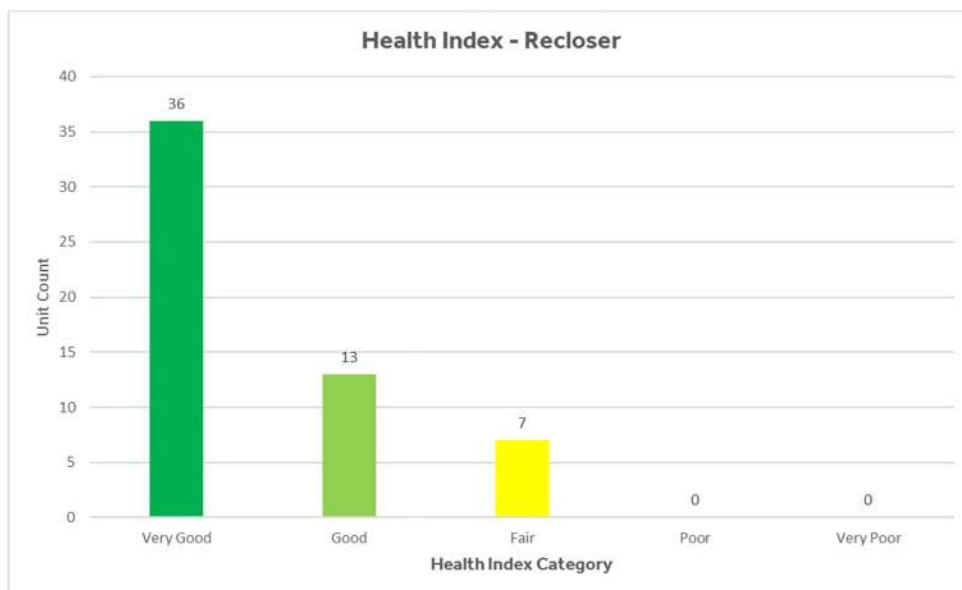
Figure 3-8: Recloser Health Index Demographic
