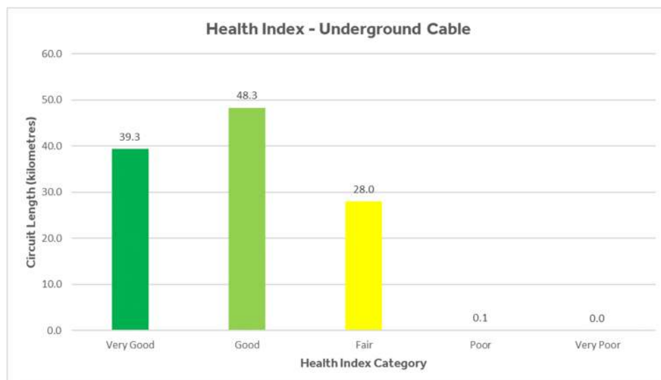
Figure 3-13: Underground Primary Cable Health Index Demographic
