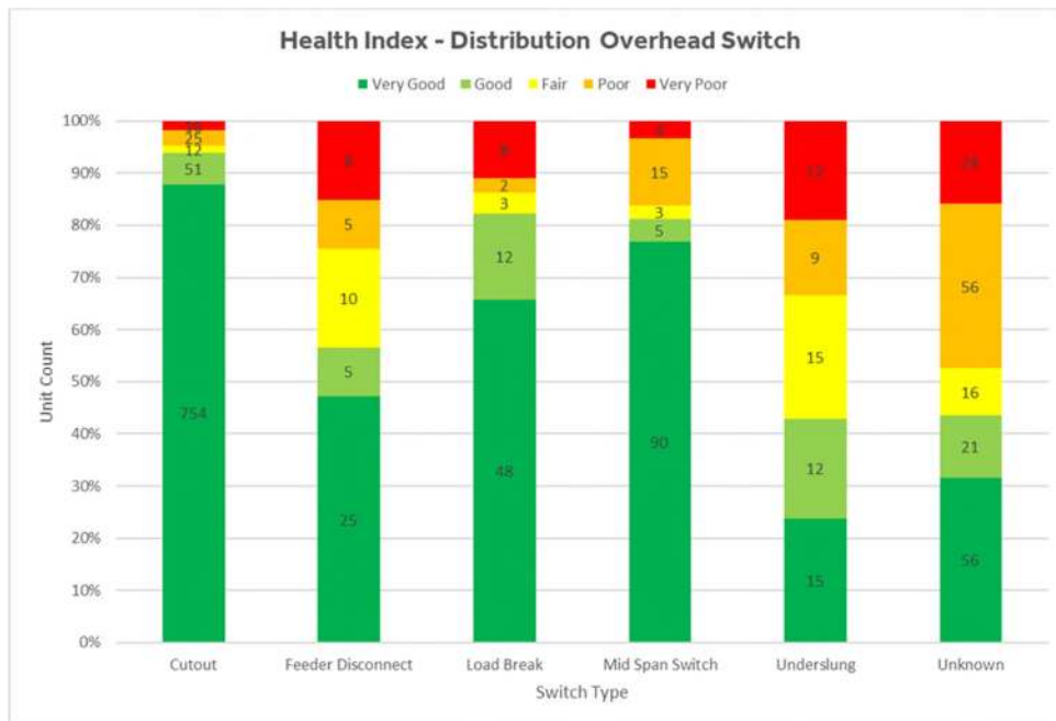
Figure 3-16: Distribution Switch Health Index Demographic
