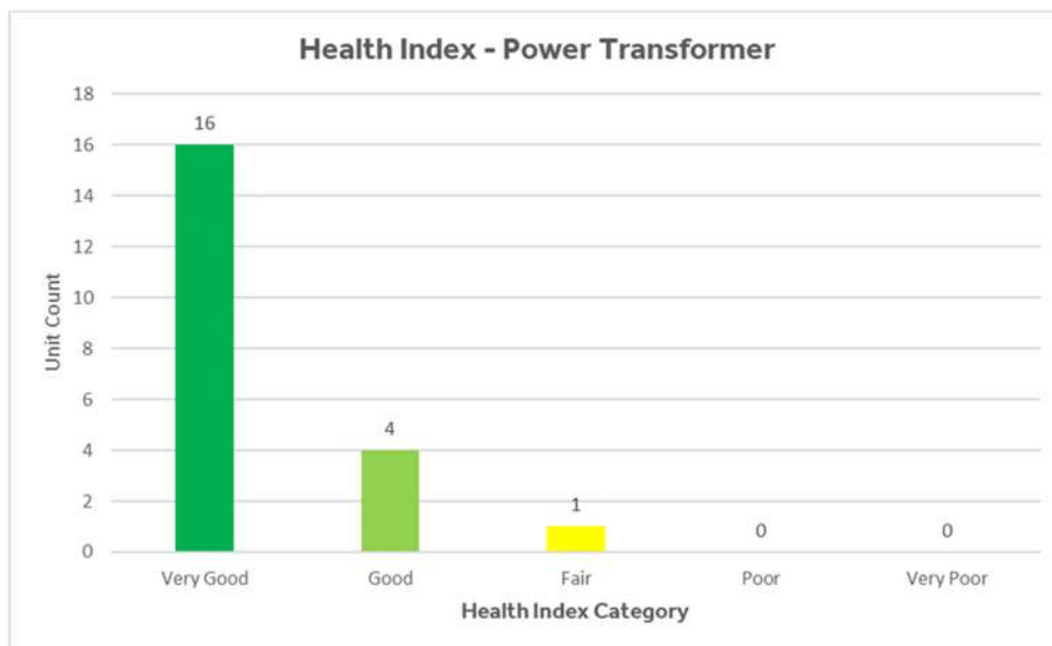
Figure 3-6: Power Transformer Health Index Demographic
