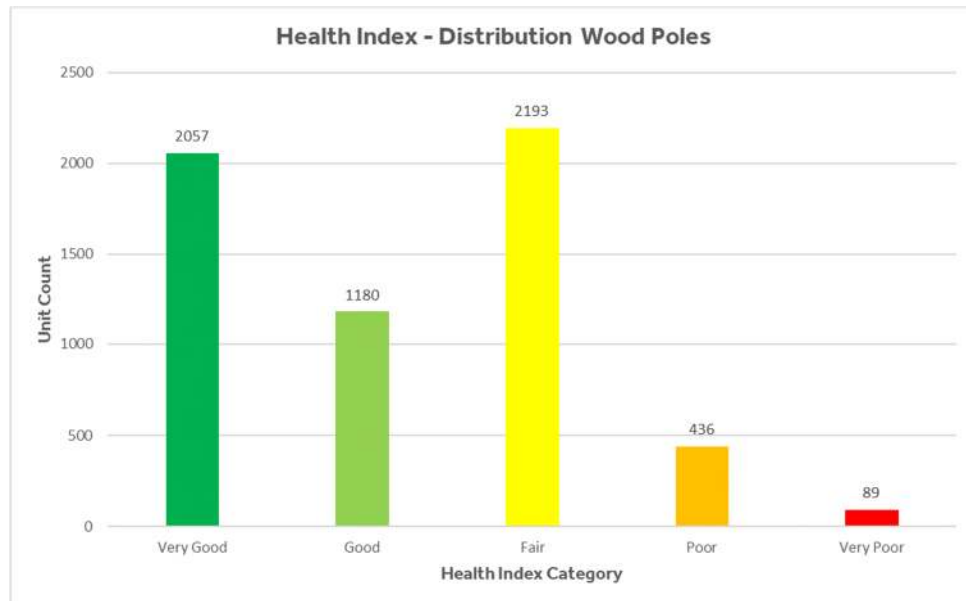
Figure 3-11: Distribution Wood Pole Health Index Demographic
