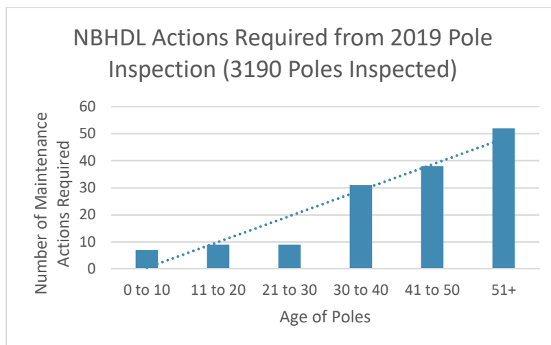
Figure 4-2 : NBHDL Actions Required from 2019 Pole Inspections
