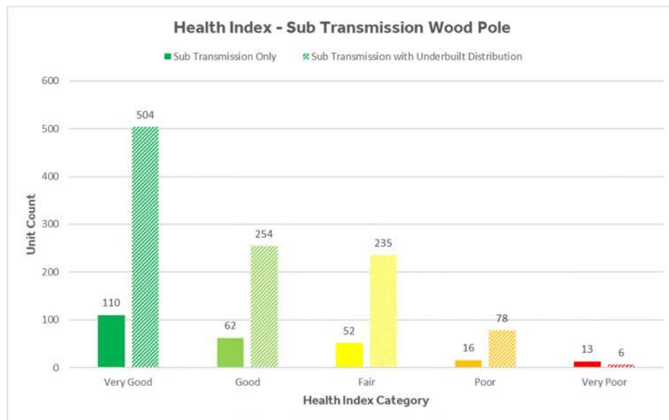
Figure 3-12: Sub-Transmission Pole Health Index Demographic
