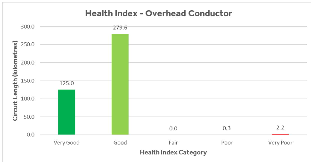
Figure 4-6: Overhead Primary Conductor Health Index Demographic
