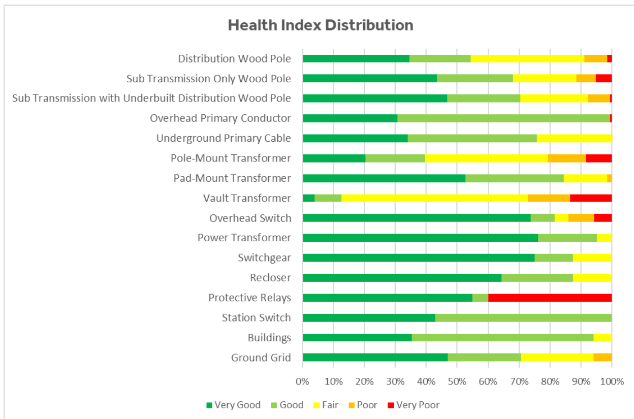
Figure 6-1: Health Index Results
